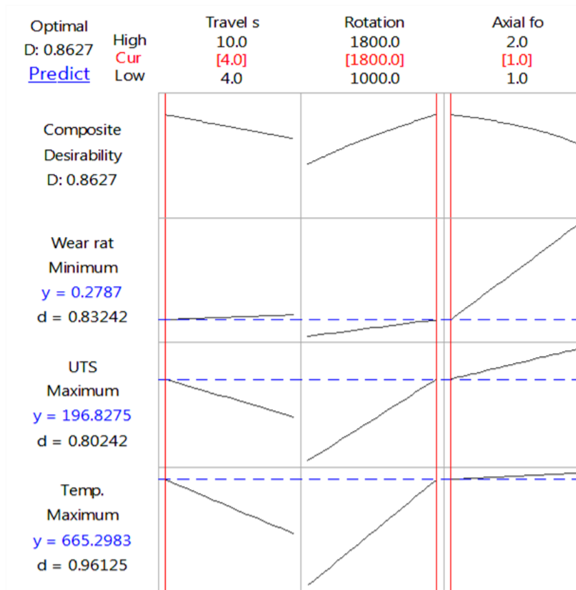
Fig. 10 A map that forecasts the ideal FSW process parameters.
