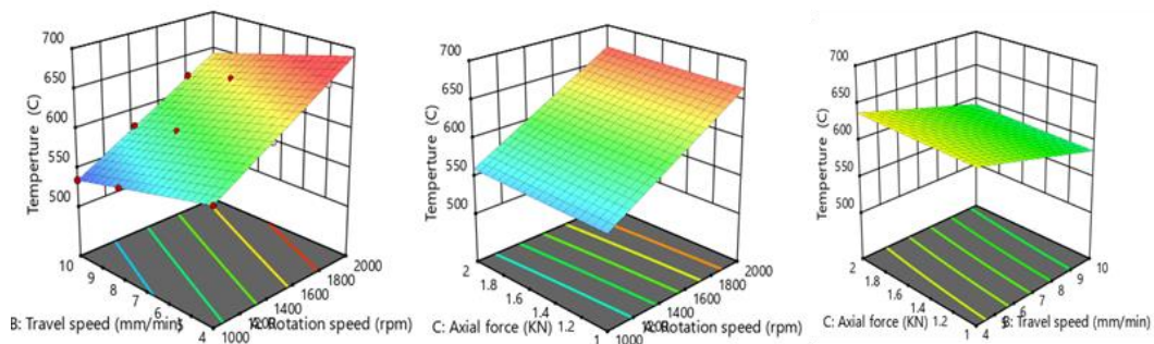
Fig. 8 Contour plots show how the axial force, weld speed, and rotation speed affect the temperature of an FSW joins.
