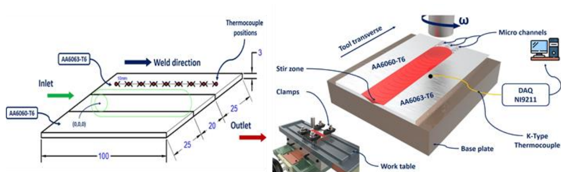
Fig. 4 (c) The position of the thermocouple.
