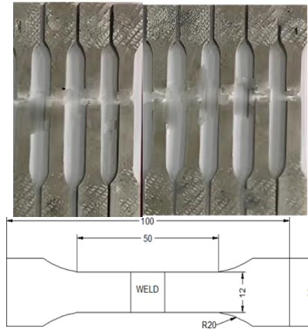
Fig. 4 (b) The tensile test specimen.
