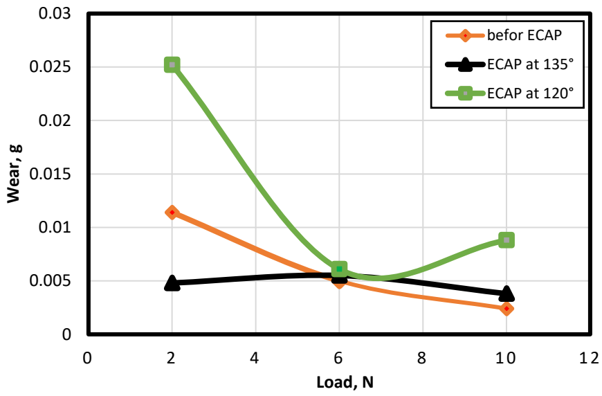
Fig. 7 Effect of angle of ECAP and applied load on the wear of Al-7075.
