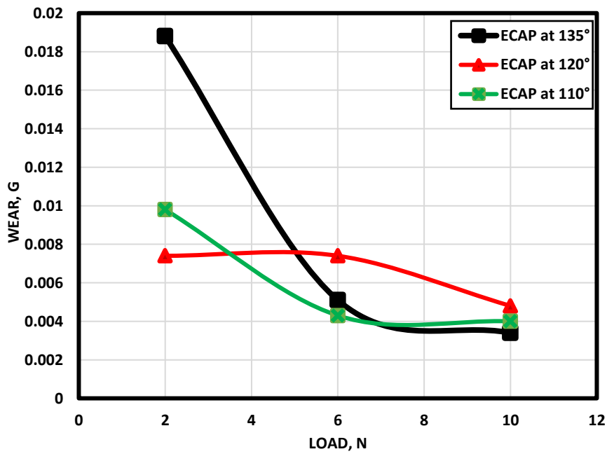
Fig. 8 Effect of angle of ECAP and applied load on the wear of Al-2021.
