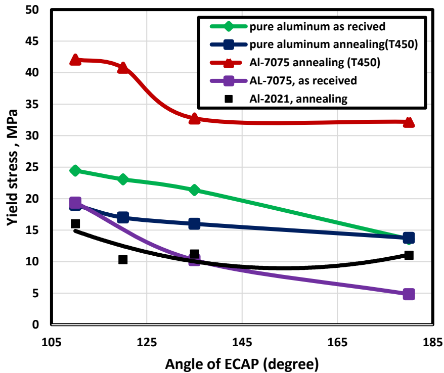
Fig. 6 Graphical representation of the variation in angles as a function of yield stress in ultra-fine grained materials.
