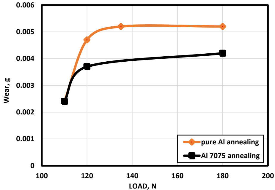
Fig. 8 Effect of type of material and applied load on the wear.
