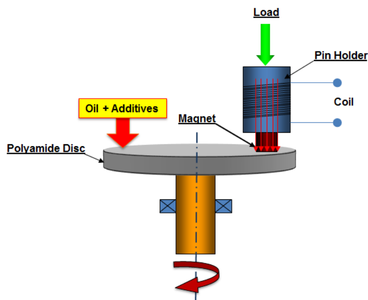
Fig. 2 Application of the magnetic field.
