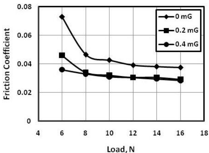
Fig. 6 Friction coefficient displayed by the sliding of steel pin against polyamide disc lubricated by oil dispersed by CMOC.
