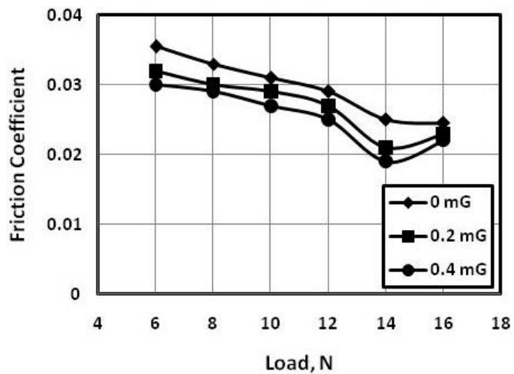
Fig. 8 Friction coefficient displayed by the sliding of steel pin against polyamide disc lubricated by oil dispersed by DA.
