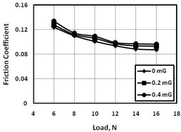
Fig. 7 Friction coefficient displayed by the sliding of steel pin against polyamide disc lubricated by oil dispersed by graphite.
