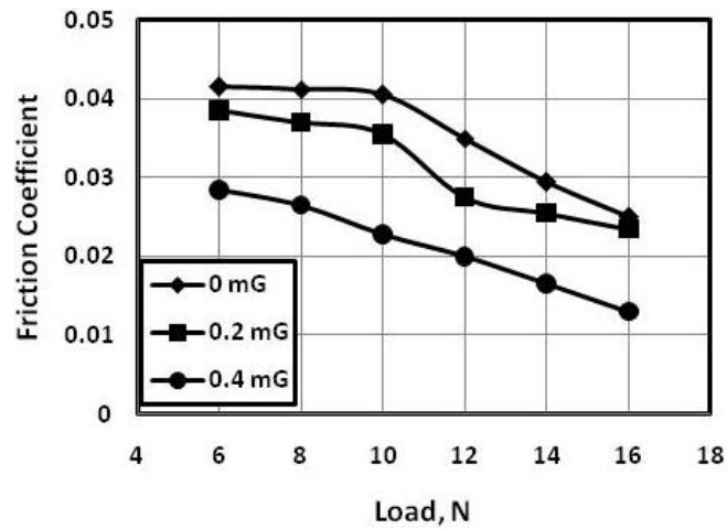
Fig. 9 Friction coefficient displayed by the sliding of steel pin against polyamide disc lubricated by oil dispersed by PTFE.
