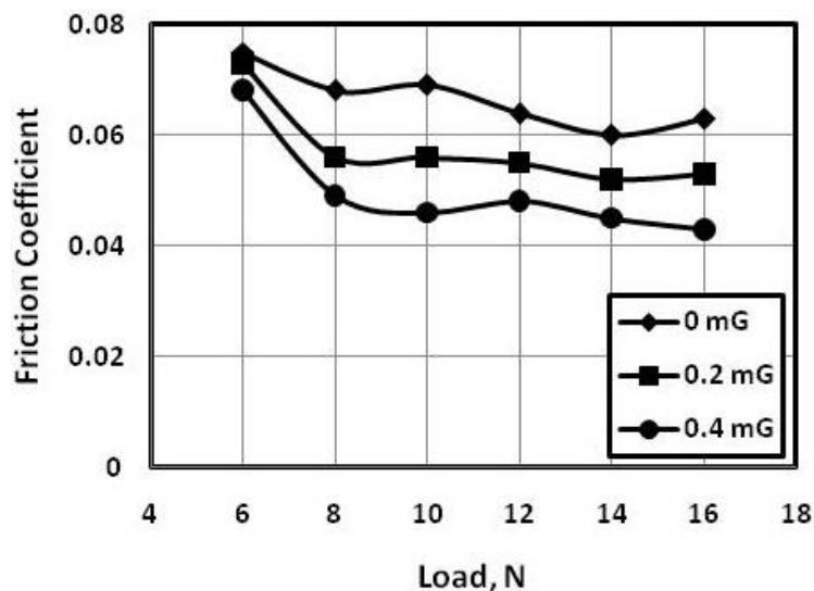
Fig. 10 Friction coefficient displayed by the sliding of steel pin against polyamide disc lubricated by oil dispersed by PMMA.
