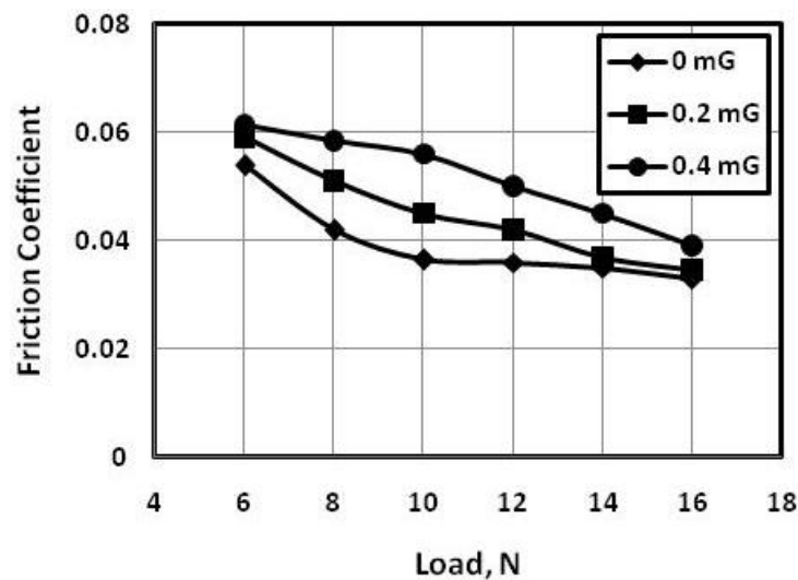
Fig. 4 Friction coefficient displayed by the sliding of steel pin against polyamide disc lubricated by oil dispersed by ZDDP.
