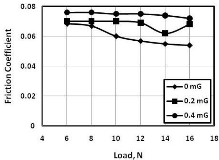
Fig. 5 Friction coefficient displayed by the sliding of steel pin against polyamide disc lubricated by oil dispersed by MoS 2 .
