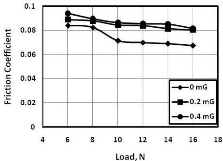
Fig. 3 Friction coefficient displayed by the sliding of steel pin against oil lubricated polyamide disc.
